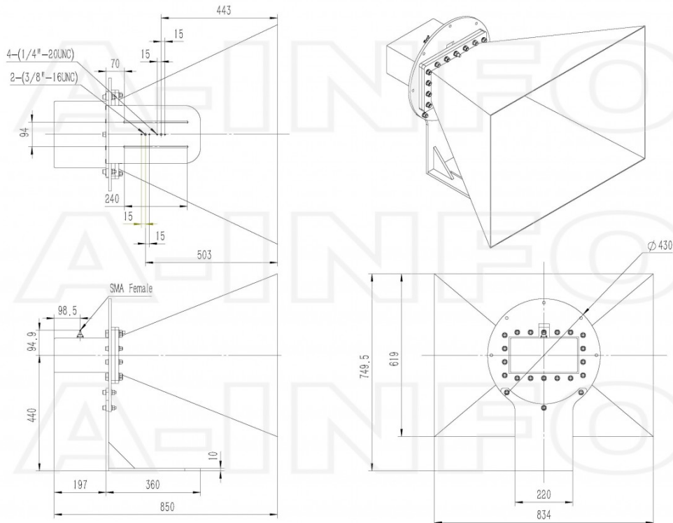
SMA Female Output with L Type Mounting Bracket (Option, P/N: LB-975-15-C-L)
