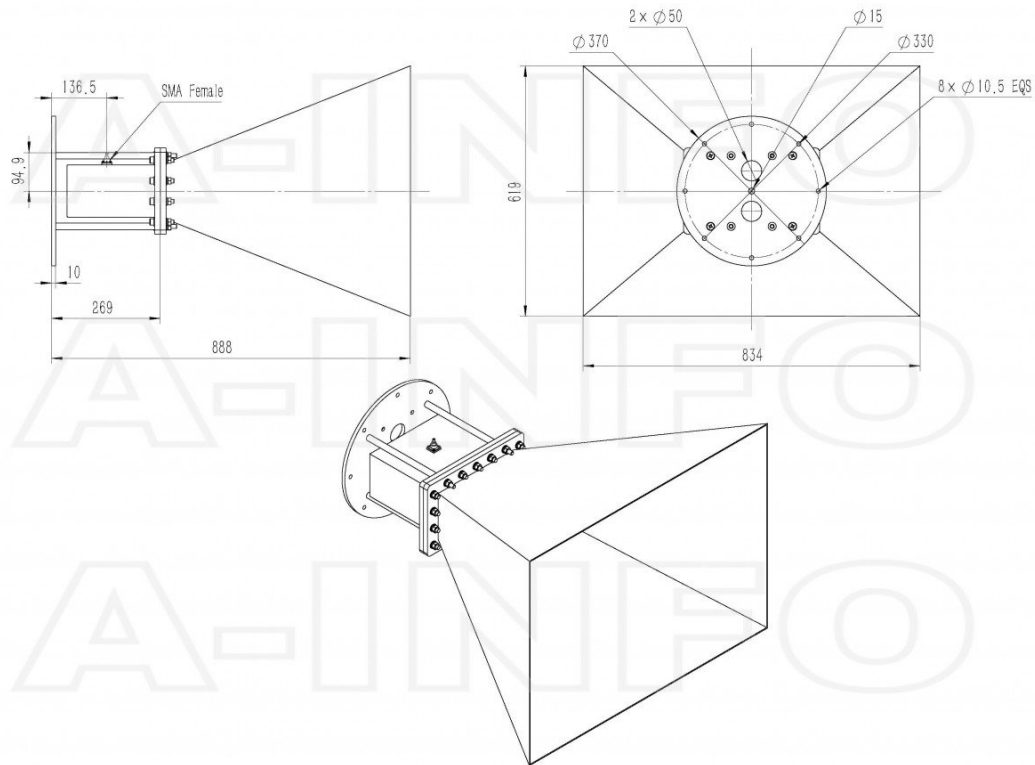
SMA Female Output with Round Mounting Bracket (Option, P/N: LB-975-10-C-MB)
